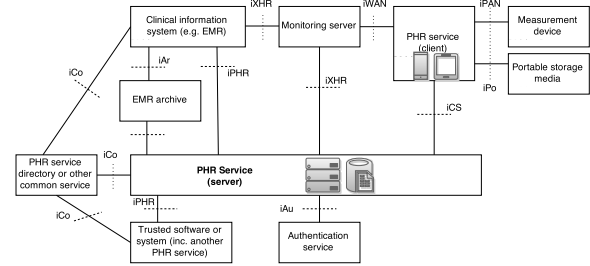
Figure 2. FeelGood reference architecture. Adapted from [10]
