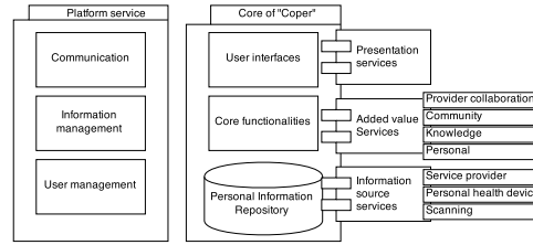
Figure 5. Coper reference architecture. Adapted from [14]
