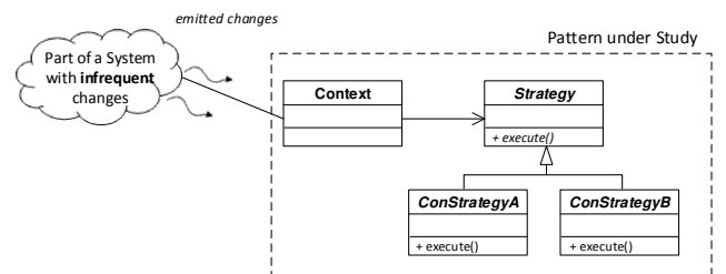
Fig. 1b Design pattern instance placed in an infrequently-changing spot of the design
